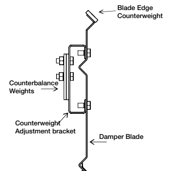
Figure 5 - Adjustable counterweight assembly detail
