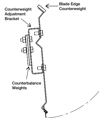
Figure 7 - Adjustable counterweight assembly detail
