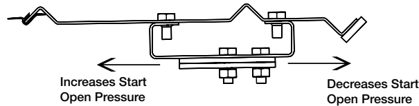
Figure 4: Counterweight adjustment for start open pressure. Blade is shown in full close position
