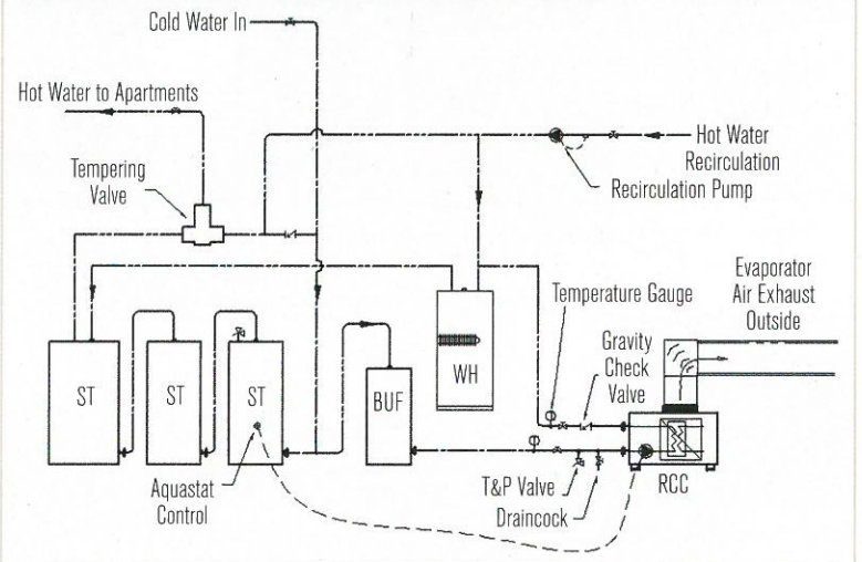
FIGURE 2 Reverse cycle chiller.
