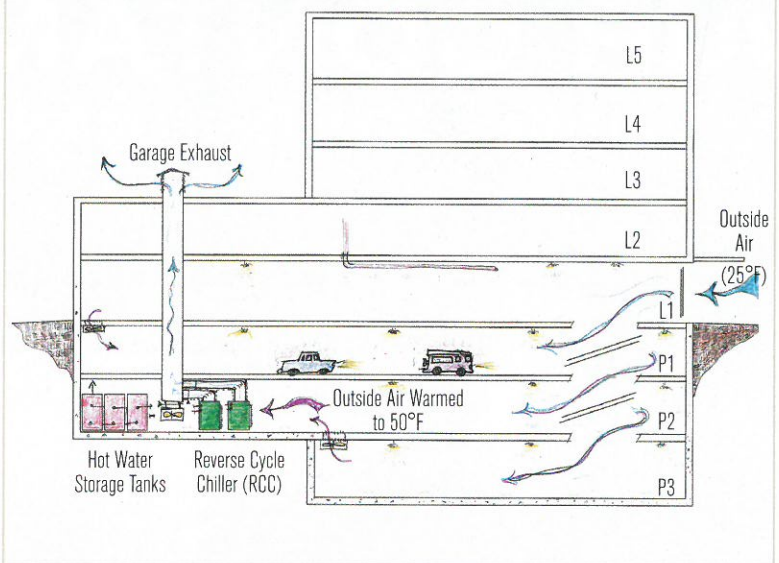
FIGURE 2 Reverse cycle chiller.
